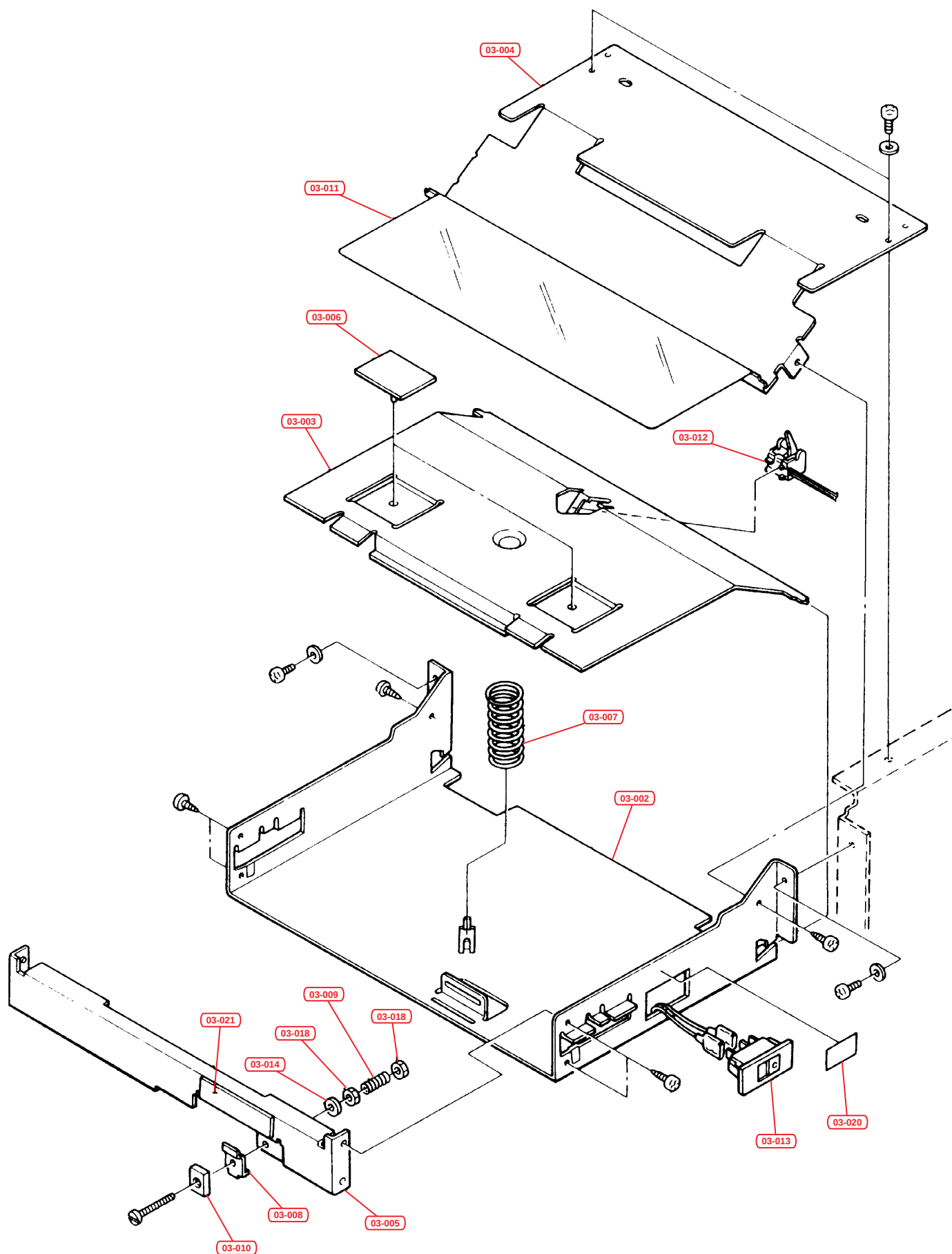
Fig.3 - Feeder Assembly
